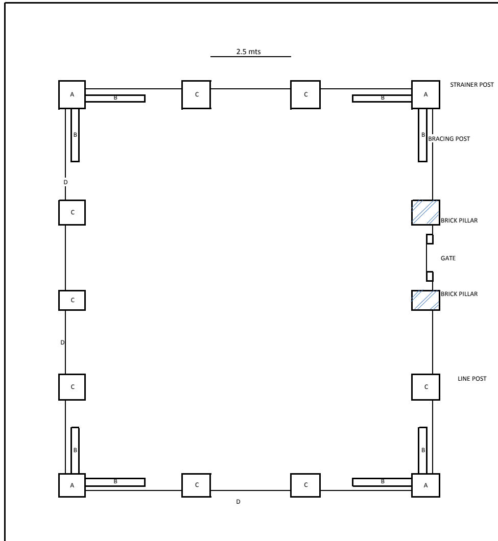
TYPICAL SCHEMATIC DIAGRAM SHOWING THE LAY OUT OF BARBED WIRE FENCING
